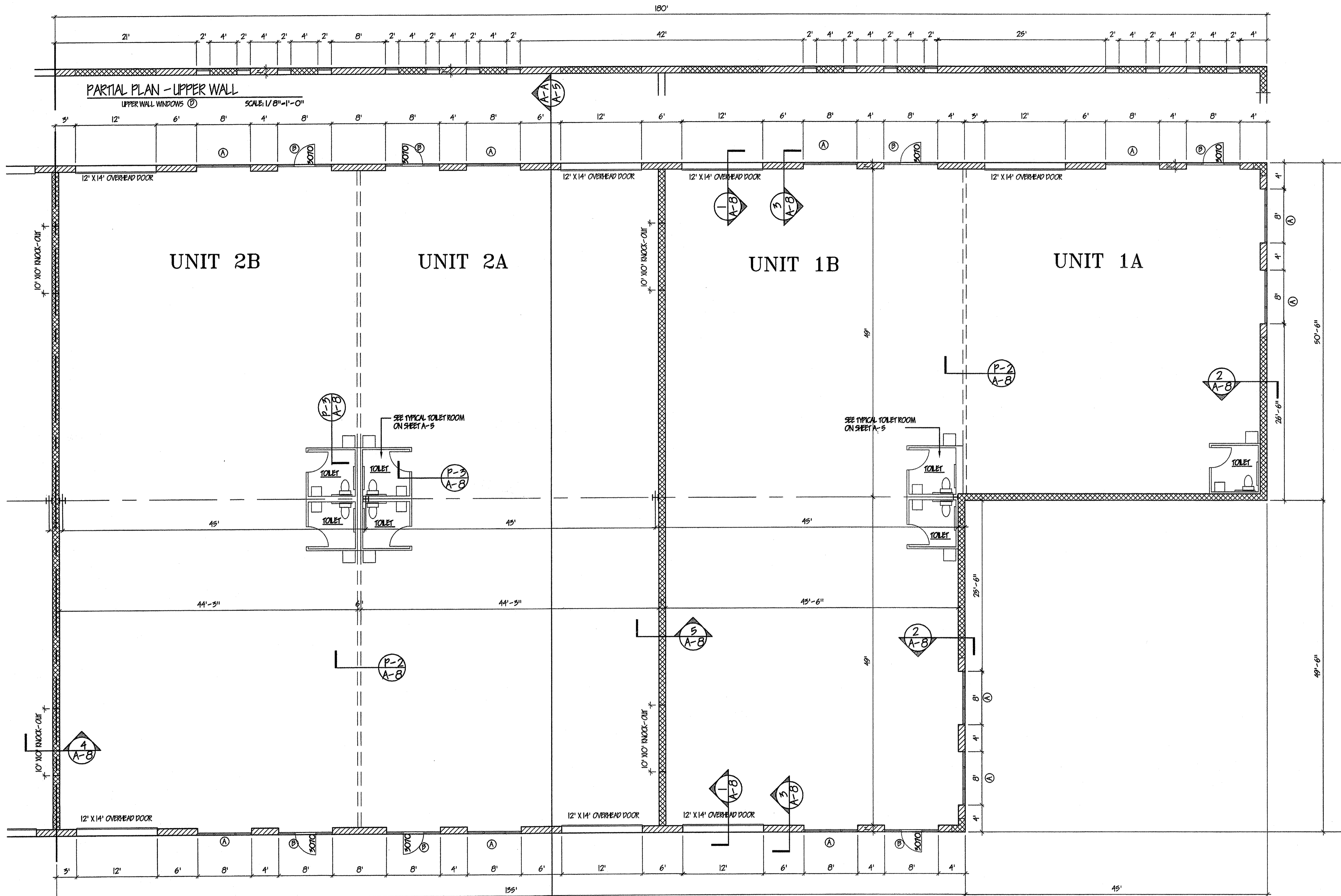
FLOOR PLAN SLAB EL. = 268.00 SCALE: 1/8"=1'-0"
