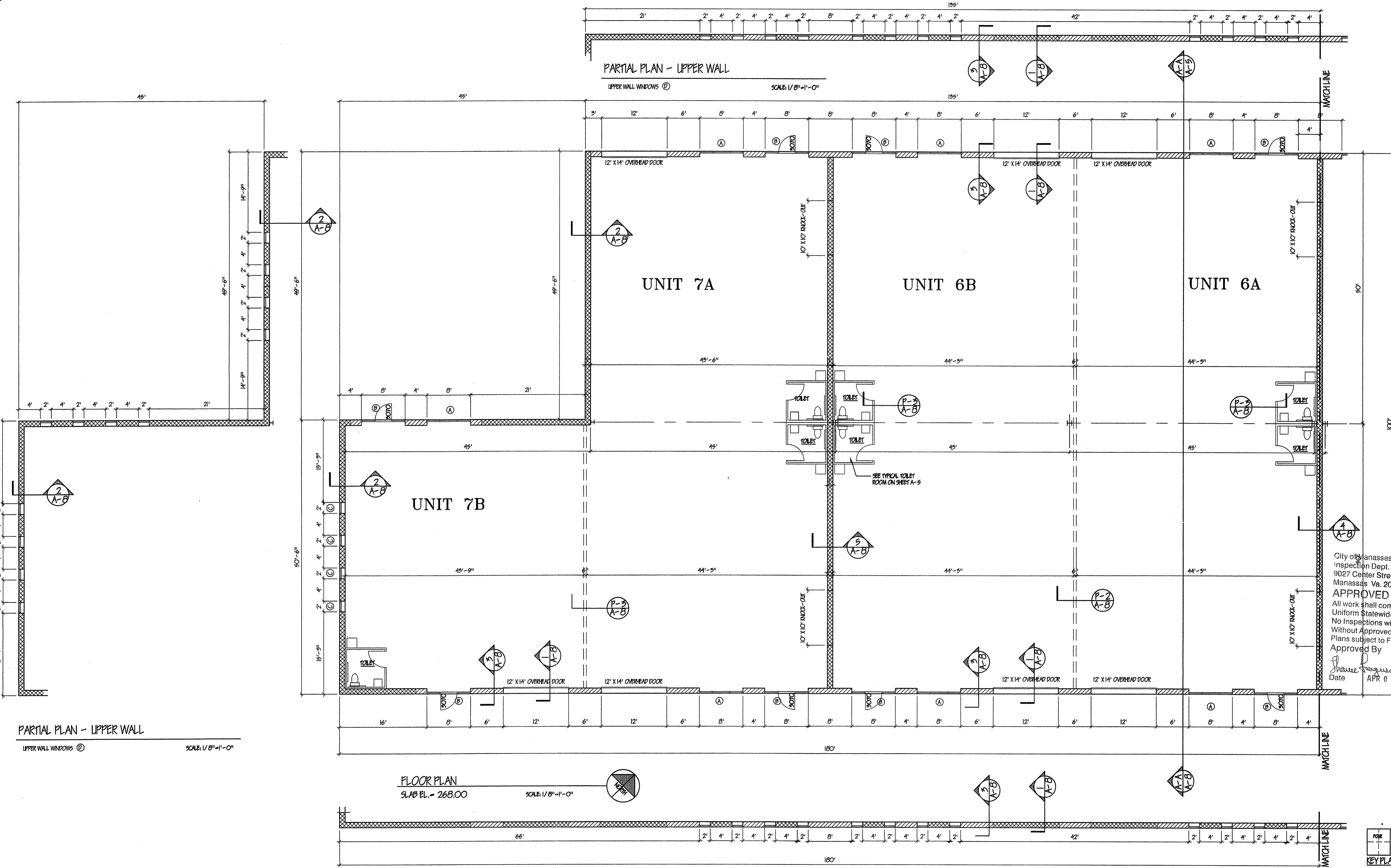
PARTIAL PLAN - UPPER WALL
